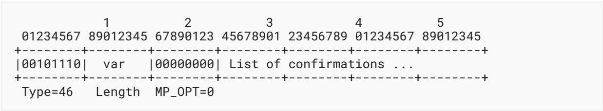
Figure 6: Format of the MP_CONFIRM Option
