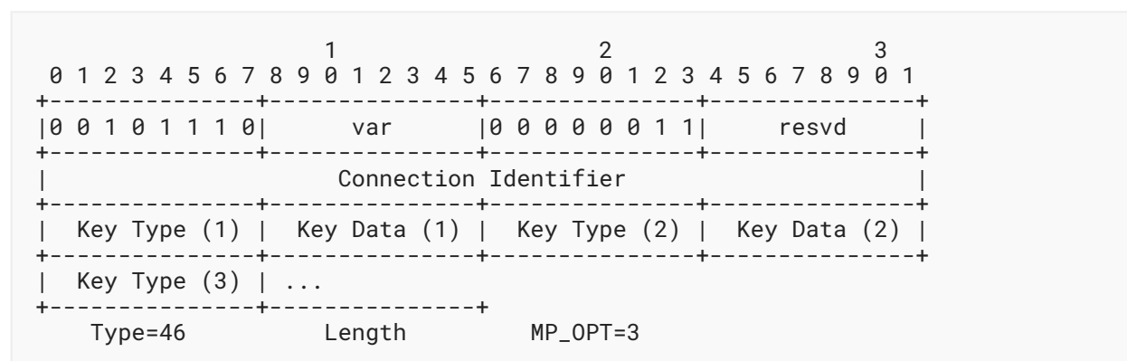
Figure 11: Format of the MP_KEY Suboption
