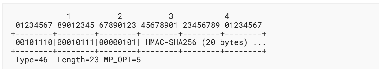
Figure 13: Format of the MP_HMAC Suboption
